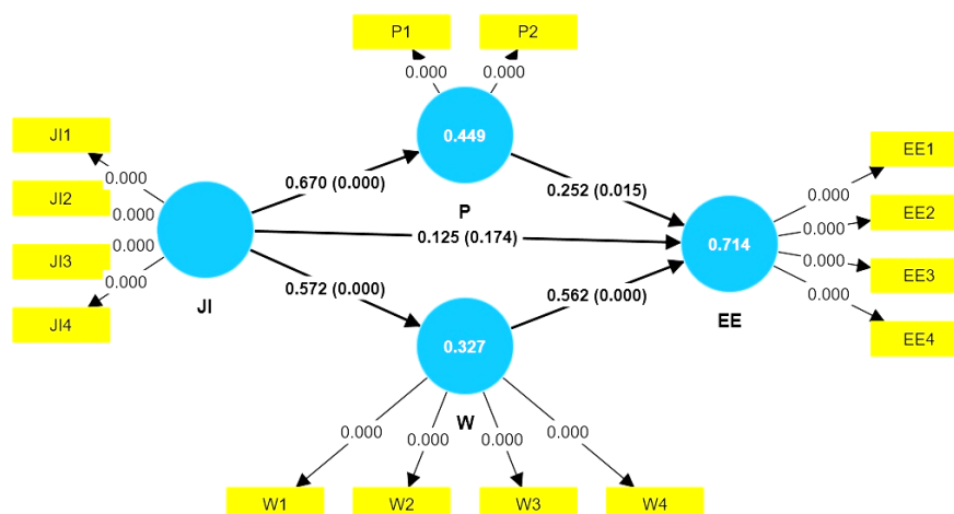
Gambar 2. Bootstrapping Test
